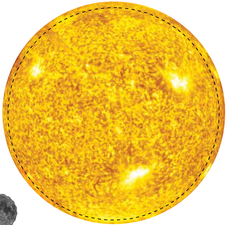
The Sun
