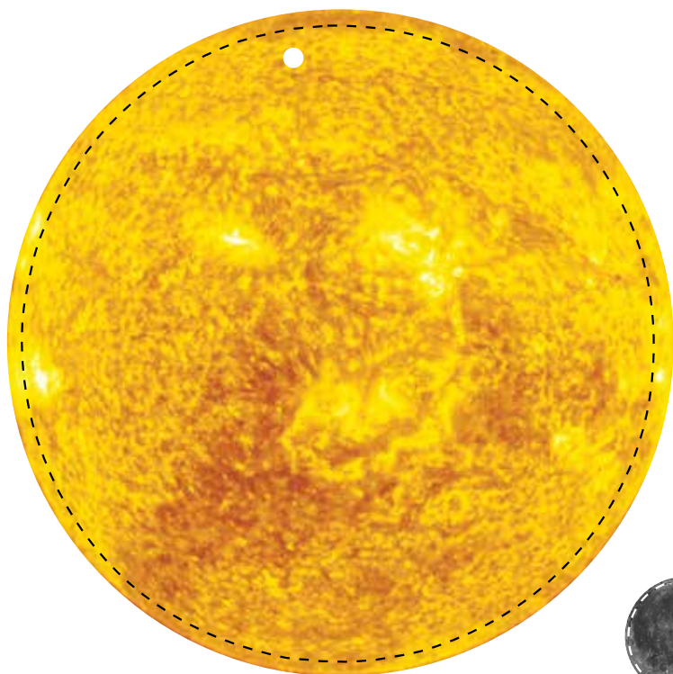
The Sun
